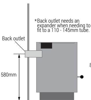
Water Tank 30 L
